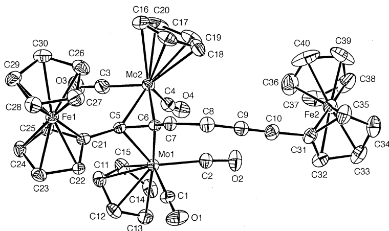
Fig. 3. ORTEP drawing of ( \mu_2 - \eta^2 - 2,2 -DFEHD)[Cp 2 Mo 2 (CO) 4 ] ( 9 ). Thermal ellipsoids are drawing in 50% probability boundaries.
