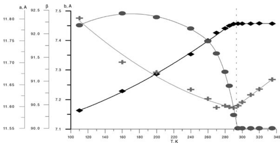
FIGURE 11 Temperature dependence of some crystall parameters in macrocycle 6a . +: a (Å); ●: angle \beta ; ◆: b (Å).
