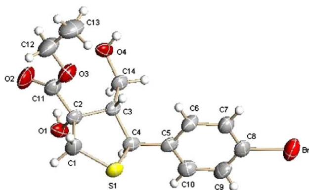
Figure 2. X-ray crystal structure of 6b .
