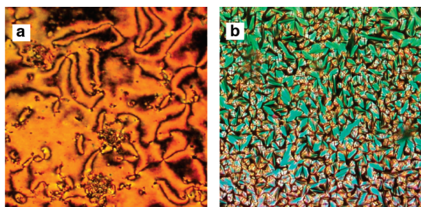
Figure 2. (a) Nematic Schlieren texture (100×) observed for 4b, obtained on cooling from isotropic liquid at 130 °C. (b) Focal-conic SmA texture (100×) observed for 4c, obtained on cooling from isotropic liquid at 120 °C.
