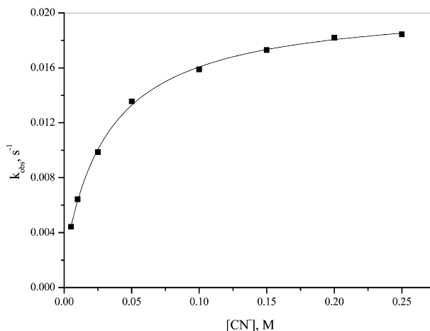
Fig. 3 Plot of k_{\text{obs}} vs. [\text{CN}^-] for the reaction between CN-13-epiCbl and \text{CN}^- at pH 11.0, 30.0 °C and I = 0.5 \text{ M} (NaClO 4 ); the solid line is a fit to eqn. (3) in the text.
