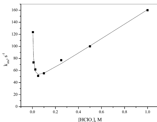
Fig. 4 Plot of k_{\text{obs}} vs. [\text{HClO}_4] for the reaction between \beta - \text{NCCH}_2 -13epiCbl and \text{HClO}_4 at 5.0^\circ\text{C} and I = 2 \text{ M} ( \text{NaClO}_4 ); the solid line is a fit to eqn. (4) in the text.
