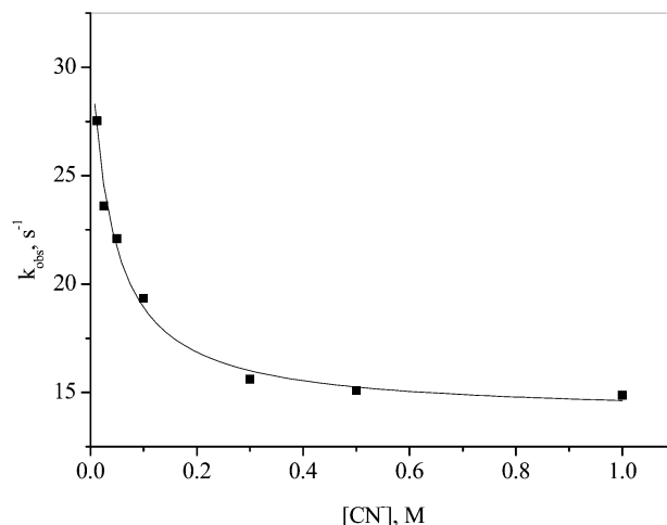
Fig. 1 Plot of k_{\text{obs}} vs. [CN − ] for the reaction between \beta -NCCH 2 -13-epiCbl and CN − at pH 11.0, 5.0 °C and I = 1.0 M (NaClO 4 ); the solid line is a fit to eqn. (3) in the text.
