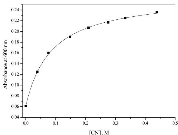
Fig. 5 Change in absorbance at 600 nm on addition of CN − to NCCH 2 -13-epiCbl; the solid line is a fit to eqn. (5) in the text and results in K_{\text{CN1}} = 13.3 \pm 1.5 \text{ M}^{-1} .
