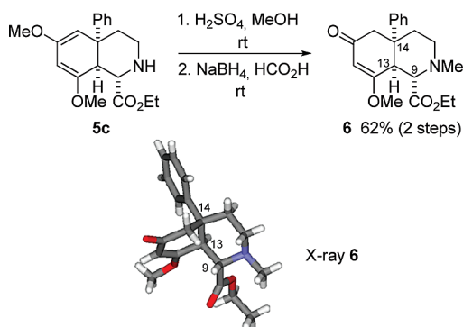
Scheme 3. Synthesis and X-ray Structure of 6
