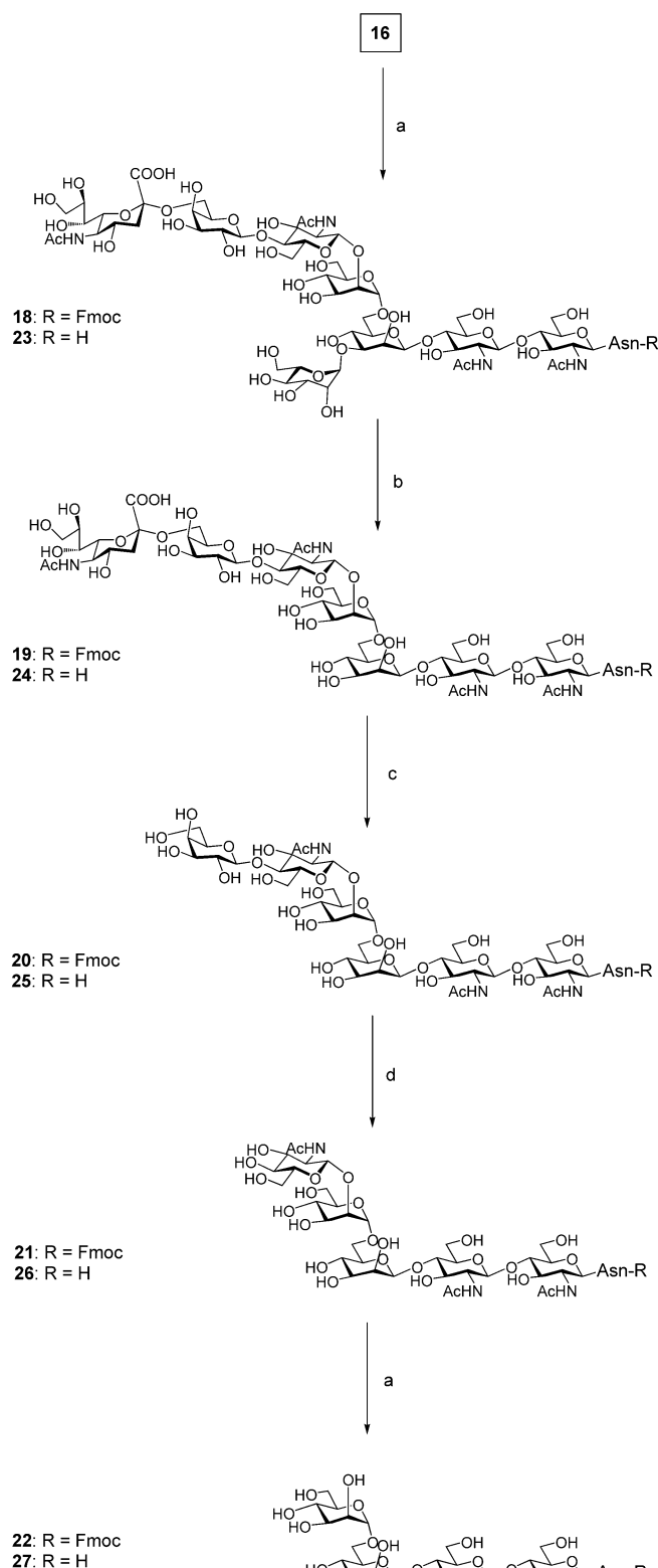
Scheme 4. a) N-Acetyl- \beta -D-glucosaminidase; b) \alpha -D-mannosidase; c) \alpha -D-neuraminidase; d) \beta -D-galactosidase.
