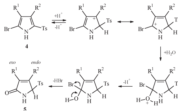
Figure 2. Acid-catalyzed conversion of \alpha -bromo- \alpha' - p -toluenesulfonylpyrroles ( 4 ) to 5- p -toluenesulfonyl-3-pyrrolin-2-ones ( 5 ). For series a : R 1 = CH 3 , R 2 = (CH 2 ) 3 CH 3 and for b : R 1 = (CH 2 ) 3 CH 3 , R 2 = CH 3 .
