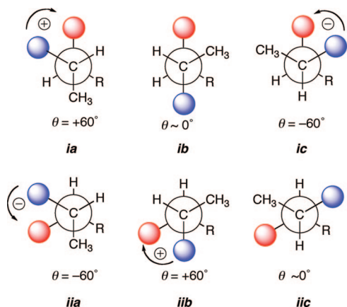
Figure 4. Staggered conformers contributing to exciton coupling CD in threo ( ia–ic ) and erythro ( iia–iic ) isomers of acyclic dibenzoyl 2-amino-3-alkanols. Blue- and red-shaded spheres represent N -Bz and O -Bz chromophore groups, respectively ( \lambda_{\text{max}} \approx 228 nm). The net signs of the observed split Cotton effects are consistent with predominant contributions from conformers ia and iia , respectively. Conformers ib and iic have antiparallel transition dipole moments and give zero contributions to the ECCDs. See also Figure 1.
