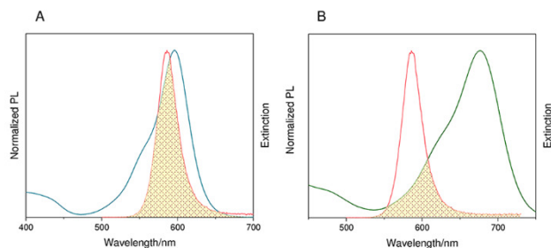
Figure 4. Normalized PL emission spectrum of EA-QDs (red line, left axis) superimposed to the extinction spectrum of (A) MASB (blue line, right axis) and (B) DASB (green line, right axis). The resulting spectral overlap integrals, J(\lambda) , are represented as shaded areas.
