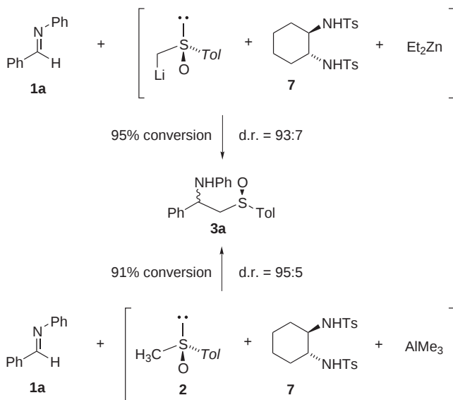
SCHEME 4 Effect of external chiral ligands (Zn and Al cations)
