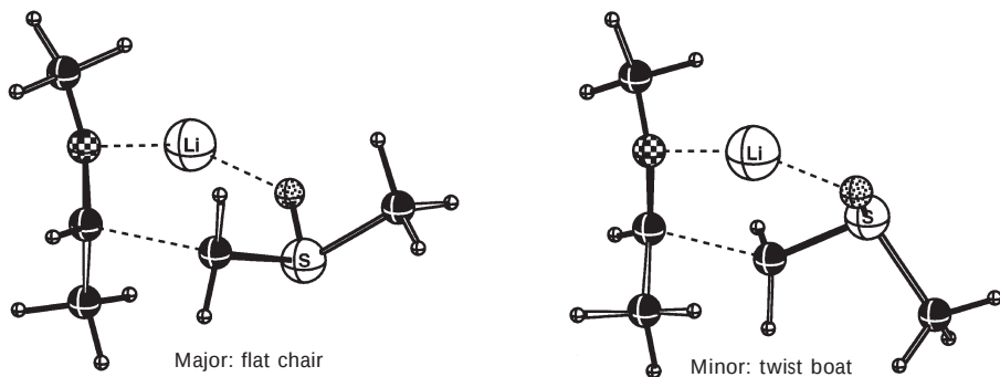
FIG. 3 Calculated diastereomeric transition states for a small model system
