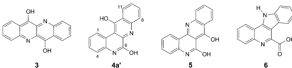
Fig. 2. Possible dibenzonaphthyridindione isomers from natural and synthetic sources: Epindolidione (3), a minor impurity in the technical indigo synthesis, and dibenzo[b,h][1,6]naphthyridine-6,7-diol (5), and 11H-indolo[3,2-c]quinoline-6-carboxylic acid (6) from Tabernanthe iboga
