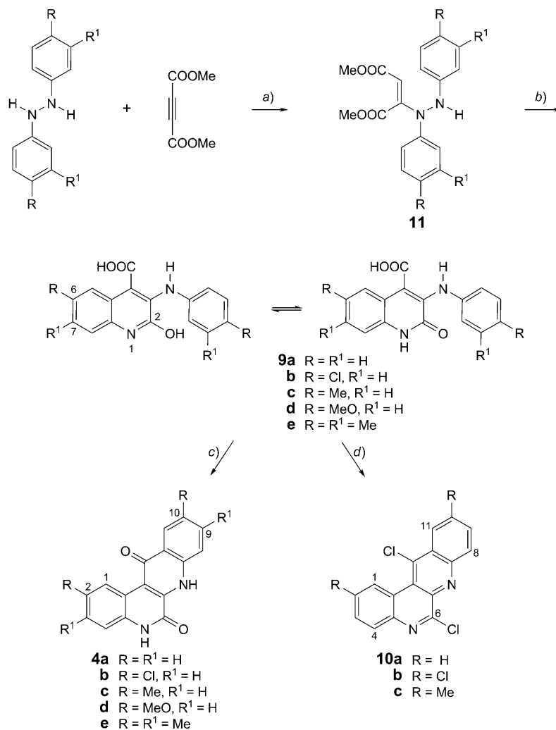
Scheme. Successful Protocol for the Synthesis of Compounds of Type 4
