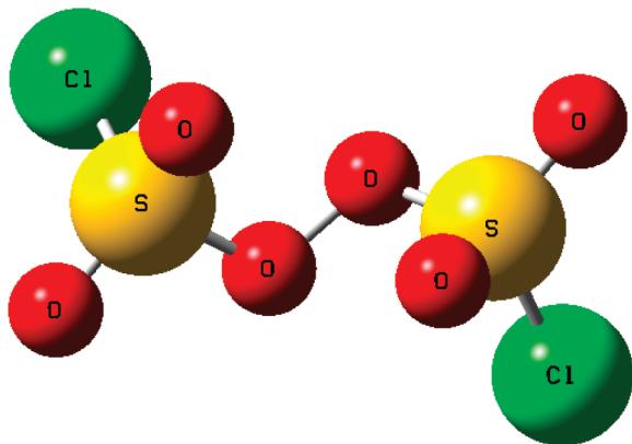
Figure 3. B3P86/6-31+G* molecular model of the most-stable conformer G^-G^- of \text{ClSO}_2\text{OOSO}_2\text{Cl} .
