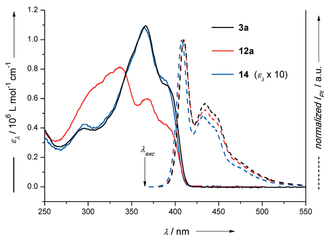
Figure 5. Quantitative UV–vis absorption spectra (continuous lines) and normalized emission spectra (dashed lines, \lambda_{\text{exc}} = 365 \text{ nm} ) of the spoked wheel ( 3a , black), the noncyclic precursor ( 12a , red), and the linear model rod ( 14 , blue, Scheme 4) in \text{CHCl}_3 . Note that 14 constitutes a suitable model chromophore both for the absorption and for the emission of the spoked wheel. See Table 2 for the molar absorption coefficients and fluorescence quantum yields.
