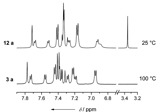
Figure 2. ^1\text{H} NMR spectra (500 MHz, \text{C}_2\text{D}_2\text{Cl}_4 ): the aromatic region of the open precursor ( 12a , 25^\circ\text{C} , top) exhibits some signals, which are masked in the better resolved high-temperature spectrum of the spoked wheel ( 3a , 100^\circ\text{C} , bottom) and vice versa. The absence of terminal acetylene signals (around \delta = 3.35 \text{ ppm} ) in the spectrum of 3a is an indication of complete cyclization. For full spectra of 3a , 3b , 12a , and 12b , see the Supporting Information.
