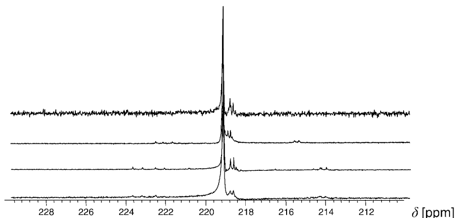
Figure. ^{13}\text{C} -NMR ( (\text{CF}_3)_2\text{C}(\text{D})\text{OD} , 125 MHz) of the poly(propene-alt-CO) copolymers prepared with the catalyst precursors [\text{Pd}(\text{P}^{\wedge}\text{P})(\text{OH}_2)_2](\text{CF}_3\text{SO}_3)_2 (see Table 1). The chelating phosphine ligands \text{P}^{\wedge}\text{P} correspond to 2 , 3a , 3b , and 3c (from top to bottom), resp.
