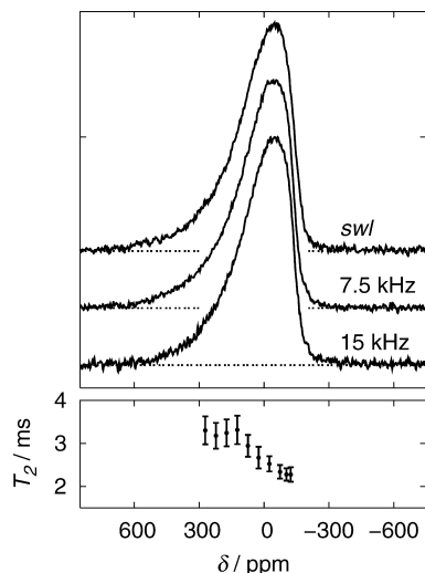
Figure 7. ^{31}\text{P} NMR signals of \text{Si}_{32.5}\text{P}_{13.2}\text{Te}_{6.6} measured at ambient temperature and B_0 = 11.74 T. The SWL and MAS signals with rotation frequencies of 7.5 and 15 kHz are normalized and separated by an arbitrary offset (top). Spin–spin relaxation time T_2 was obtained from frequency-dependent selective excitation experiments (bottom).
