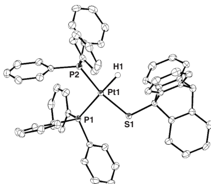
Figure 2. ORTEP drawing of 5 (30% thermal ellipsoids). Two solvated CH 2 Cl 2 molecules and hydrogen atoms are omitted for clarity. Selected bond lengths (Å) and angles (deg): Pt1–S1 = 2.3172(12), Pt1–H1 = 1.684(10), Pt1–P1 = 2.3411(12), Pt1–P2 = 2.2511(12), S1–Pt1–H1 = 88(2), P1–Pt1–P2 = 103.25(4), P1–Pt1–S1 = 90.51(4), P2–Pt1–H1 = 78(2), P2–Pt1–S1 = 165.75(4), P1–Pt1–H1 = 178(2).
