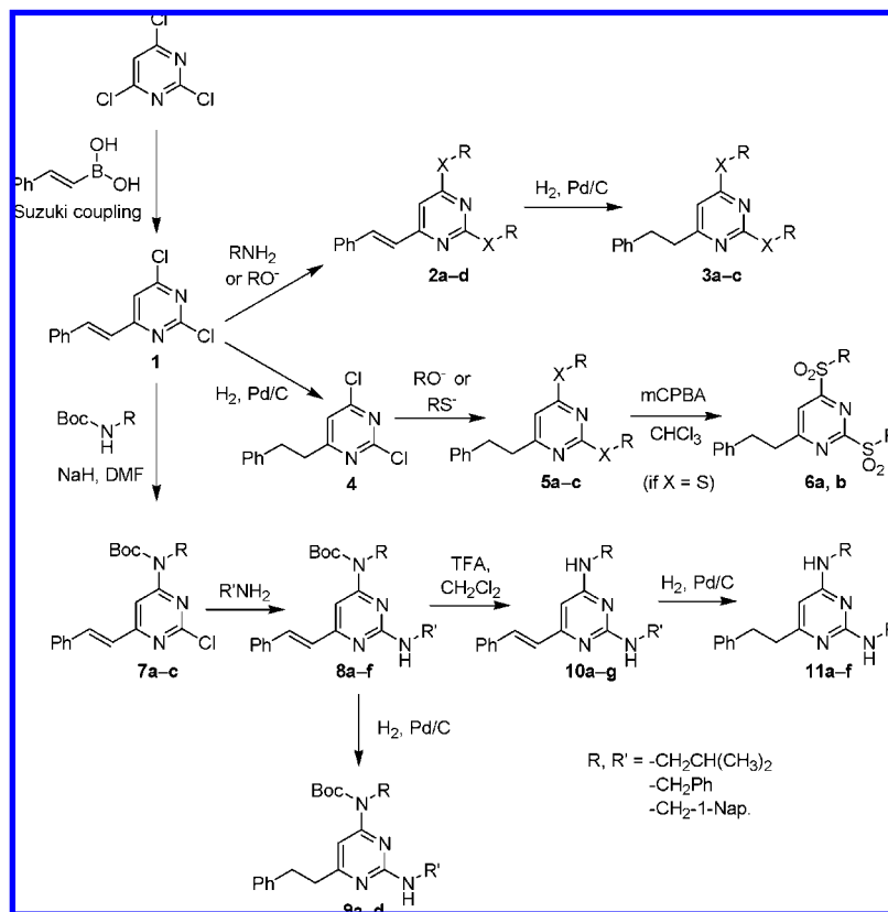
Scheme 1. Synthesis of “Symmetric” and Unsymmetric 2,4-Diamino-6-phenethylpyrimidines
