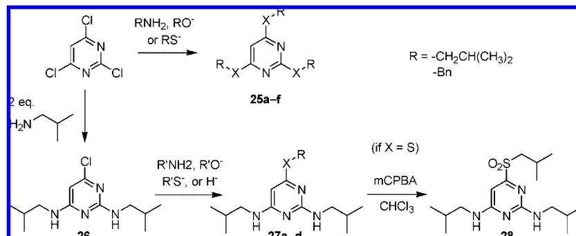
Scheme 5. Synthesis of N -Methylated Pyrimidines
