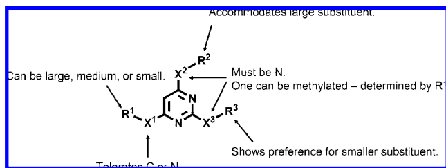
Figure 4. Summary of the structure–activity relationships of the pyrimidine-core CBIs.
