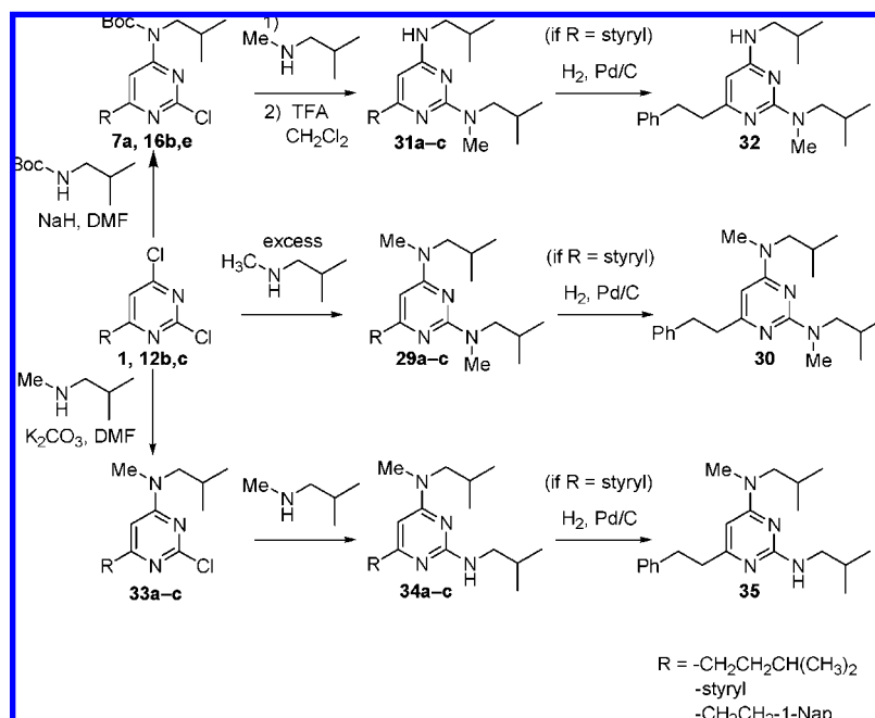
Scheme 6. Synthesis 2-Alkoxy, 2-Sulfanyl, and 2-Sulfonylpyrimidines
