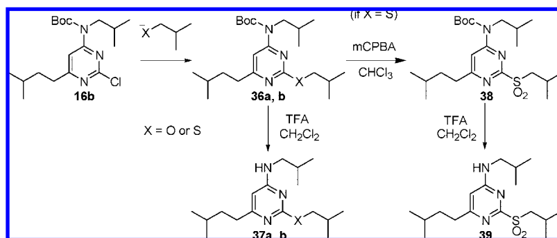
Scheme 6. Synthesis 2-Alkoxy, 2-Sulfanyl, and 2-Sulfonylpyrimidines
