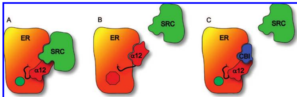
Figure 1. Cartoon representation of classical vs CBI antagonism of ER. (A) Conformation of agonist-bound ER with helix 12 forming part of the steroid receptor coactivator (SRC) binding site. (B) Conformation of antagonist-bound ER in which helix 12 occupies the SRC binding site, disrupting the ER–SRC interaction indirectly. (C) Conformation of agonist-bound ER in which a CBI occupies the SRC binding site, disrupting the ER–SRC interaction directly.
