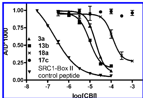
Figure 3. In vitro coactivator binding inhibition assay. TR-FRET assay shows displacement of SRC-3-NRD-F1 by control peptide and pyrimidine CBIs.
