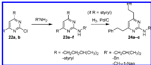
Scheme 3. Synthesis of 4,6-Dialkyl-2-aminopyrimidines
