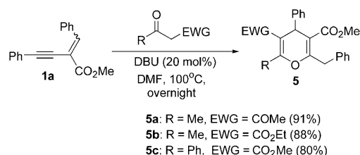
Scheme 4. DBU-catalyzed formal [3+3] cycloaddition of β-keto compounds with 1a .
