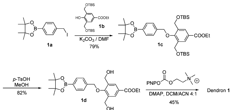
Scheme 1. Chemical Synthesis of Dendron 1
