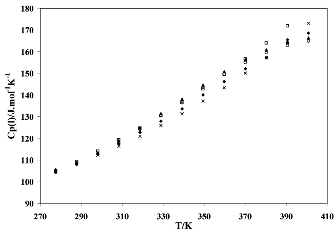
Figure 2. Comparison of liquid phase heat capacities for ethanol. ♦, this work; □, ref 10; ▲, ref 26; ○, ref 28; ×, ChemCad v5.2.
