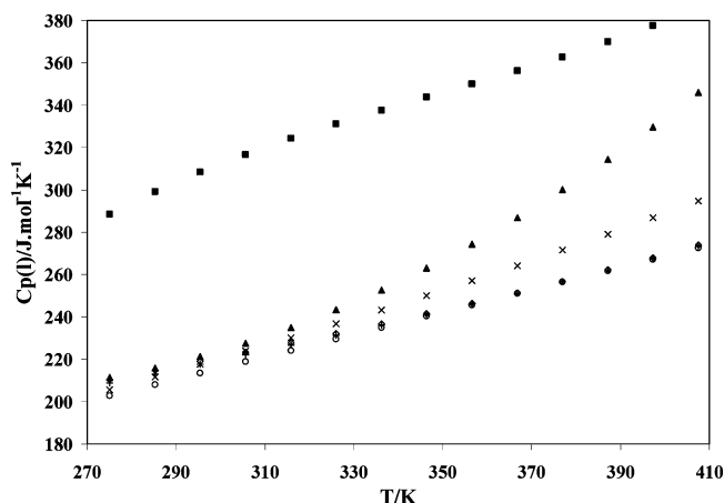
Figure 3. Comparison of liquid phase heat capacities for ETBE. ◇, This work; ■, ref 33; +, ref 26; ×, ref 10; ▲, ref 13; ○, ChemCad v5.2.
