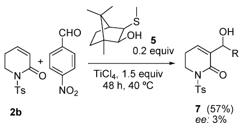
Scheme 2. MBH Reaction of 2b with p -Nitrobenzaldehyde
