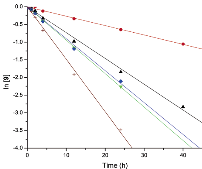
FIGURE 13. Pseudo-first-order hydrolysis kinetics for compound 9 at 37 °C: ●, pH 4.6; ▲, pH 5.7; ▼, pH 6.9; ◆, pH 7.4; +, pH 8.9.
