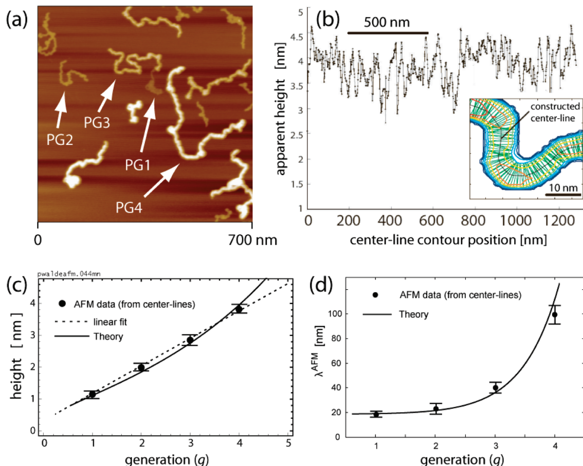
Figure 8. (a) AFM height image of a mixture of PG1 1000 –PG4 1000 spin-coated from chloroform onto mica showing mainly individual entities. Representative chains of each generation are marked. For data collection and analysis larger images ( 1.5\ \mu\text{m} \times 1.5\ \mu\text{m} ) were used. (b) Determination of an apparent height profile of a PG4 1000 chain using a tool that recognizes chains and their closed envelopes, thus ignores the background, and allows studying height profiles of single chains, like the one shown, in detail (see ref 39). The inset is a zoom into the contour plot of a region of a dendronized polymer. Lines generally follow equidistant heights. The green lines, however, are perpendicular to the center-line and are calculated by searching for spatially nearest neighbors on same contour lines, separated by at least one-third of the size of the whole polymeric object. The “center-line” connects adjacent middle points of the green lines. Its coordinates allow extracting heights along the centerline. (c) Apparent heights of PG1 1000 –PG4 1000 versus generation. The straight dotted line is a least-squares linear fit. Since the AFM measurements were carried out in the air, on dry samples, the thickness of the chains is expected to correspond to the collapsed state of the side chains when r^2\delta \approx v_{\text{monomer}}n leading in the case of X = 3 to r \approx (v_{\text{monomer}}/\delta)^{1/2}(2^g - 1)^{1/2} (solid line). For the range considered this expression is close to the observed linear dependence though deviations are expected at higher generations. (d) “AFM persistence length” of the adsorbed chains versus generation. Solid line is using eq 11.
