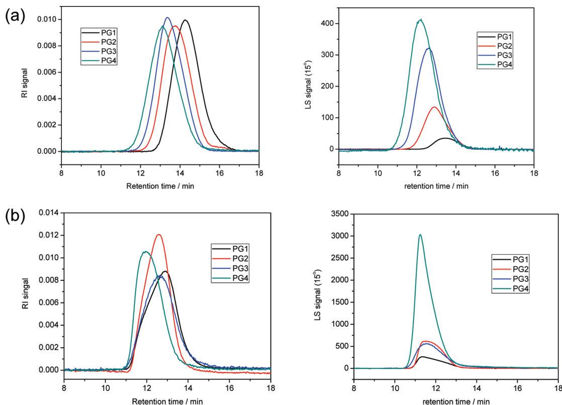
Figure 5. GPC elution curves based on refractive index (left) and Light Scattering (LS) detection at 15° scattering angle (right) of the homologous series (a) PG1 1000 – PG4 1000 and (b) PG1 7000 – PG4 7000 . All elution curves of one set belong to one and the same homologous series. All measurements were done in DMF (1% LiBr) at 45 °C.
