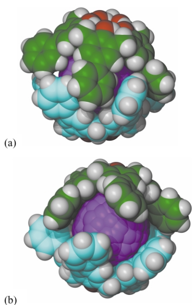
Fig. 2 Space filling projections of the molecular capsules in [C 60 ⊂ (1) 2 ].
