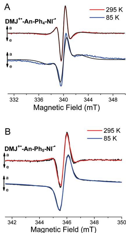
Figure 9. TREPR spectra of (A) DMJ + -An-Ph 4 -NI - at 300 ns, (B) DMJ + -An-Ph 5 -NI - at 400 ns, following a 416 nm, 1.5 mJ laser pulse at the indicated temperatures in toluene. Smooth curves superimposed on the experimental spectra are computer simulations of the radical pair spectra (see text) with the parameters given in Table 2. Positive features are in enhanced absorption, while negative features are in emission.
