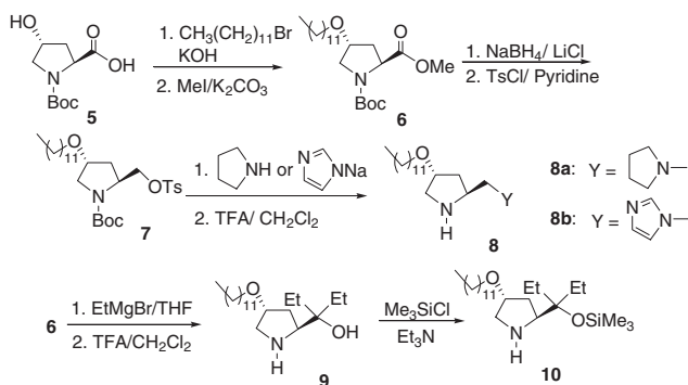
Scheme 1. Synthesis of pyrrolidine organocatalysts bearing long chain 8 – 10 .
