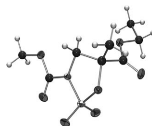
Figure 1. X-ray structure of sulfamate ( R )- 1c .
