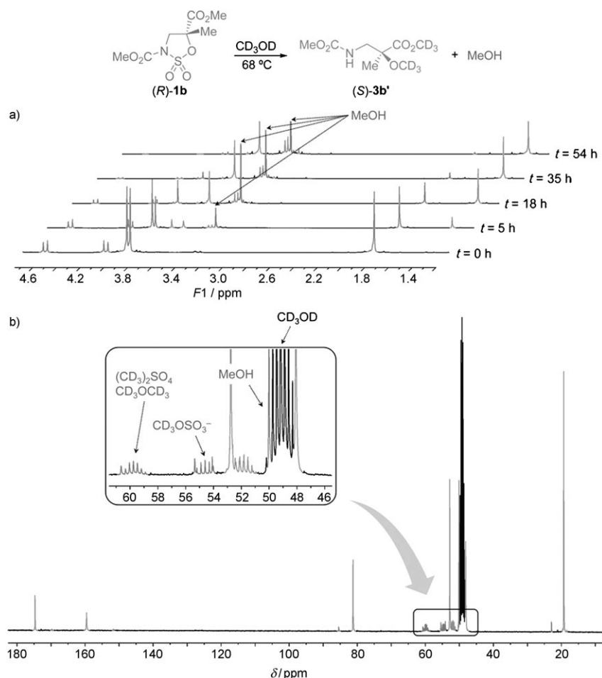
Figure 3. Reaction of sulfamidate ( R )- 1b with CD 3 OD monitored by NMR spectroscopy. a) The stacked 1 H NMR spectra show the clean and direct conversion of ( R )- 1b into ( S )- 3b' and the simultaneous (but faster) disappearance of the ester signals in both the reactant and the product (CO 2 Me, δ = 3.89 and 3.75 ppm, respectively) due to transesterification with CD 3 OD (with the subsequent evolution of MeOH). As a consequence, a slight growing of the ether signal (OCH 3 , δ = 3.31 ppm) arising from the competitive ring opening with the generated MeOH is also appreciated. b) The 13 C NMR spectrum shows the presence of small amounts of deuterated dimethyl ether and sulfonic derivatives at the end of the reaction.
