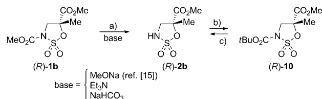
Scheme 7. Deprotection/protection of hindered sulfamides under basic conditions. a) MeOH, 68 °C, 48 h (81–93 % conv.); b) Boc 2 O, Et 3 N, CH 2 Cl 2 , 25 °C, 32 h (76 %); c) MeOH, 68 °C, 48 h (72 % conv.).
