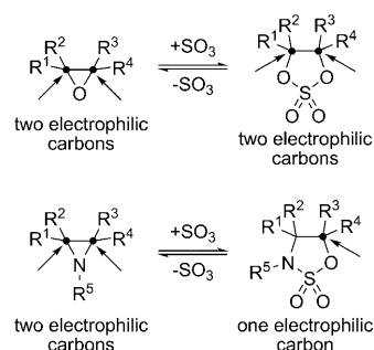
Scheme 1. Interconversions of epoxides-sulfates and aziridines-sulfamides. The reactive positions of each substrate (apart from sulfur atom) are shown with arrows.
