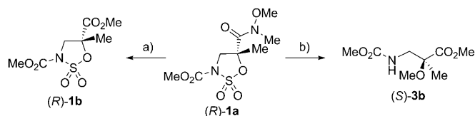
Scheme 4. Sequential and one-pot ring-opening reactions of sulfamate ( R )- 1a (optimized conditions). a) MeOH, TfOH (1.5 equiv), 40 °C, 24 h (98%); b) MeOH, TfOH (1.5 equiv), 68 °C, 48 h (98%).
