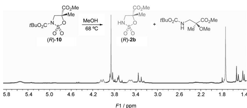
Figure 2. Reaction of sulfamide ( R )- 10 with methanol after 48 h at reflux. The 1 H NMR spectrum of the crude mixture shows the clean cleavage of the carbamate group in the sulfamide together with a small amount of the N-protected ring-opening product (the conformational isomerism of the Boc group is revealed in some duplicated signals).
