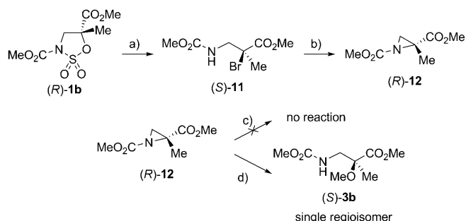
Scheme 9. Synthesis and ring-opening reaction of sulfamidate-derived aziridine ( R )- 12 . a) i) Bu 4 NBr, CH 3 CN, 25 °C, 20 h; ii) 20% H 2 SO 4 /CH 2 Cl 2 1:1, 25 °C, 8 h (76 %); b) t BuOK, THF, 0 °C, 12 h (43 %, unoptimized conditions); c) MeOH, 68 °C, 48 h; d) MeOH, p TsOH·H 2 O (1.0 equiv), 68 °C, 48 h (86 % conv., ee > 93 % determined by GC analysis, see the Supporting Information).
