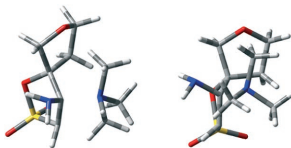
Figure 6. Geometry of the intermediate state resultant of the interaction between 41 and \text{NMe}_3 .
