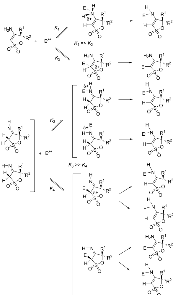
Scheme 9. Electrophilic reactions of \beta -amino- \gamma -sultone derivatives and their corresponding tautomers.
