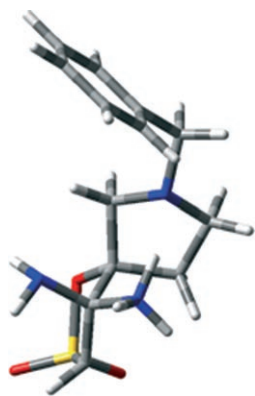
Figure 4. Molecular model of the resultant intermediate ( I ) of the reaction between 41 and \text{NH}_3 .
