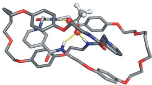
Fig. 3 Lowest energy structure of 1^{2+}\text{CH}_3\text{CO}_2^- , obtained by gas phase simulated annealing molecular dynamics. Details as in Fig. 2.
