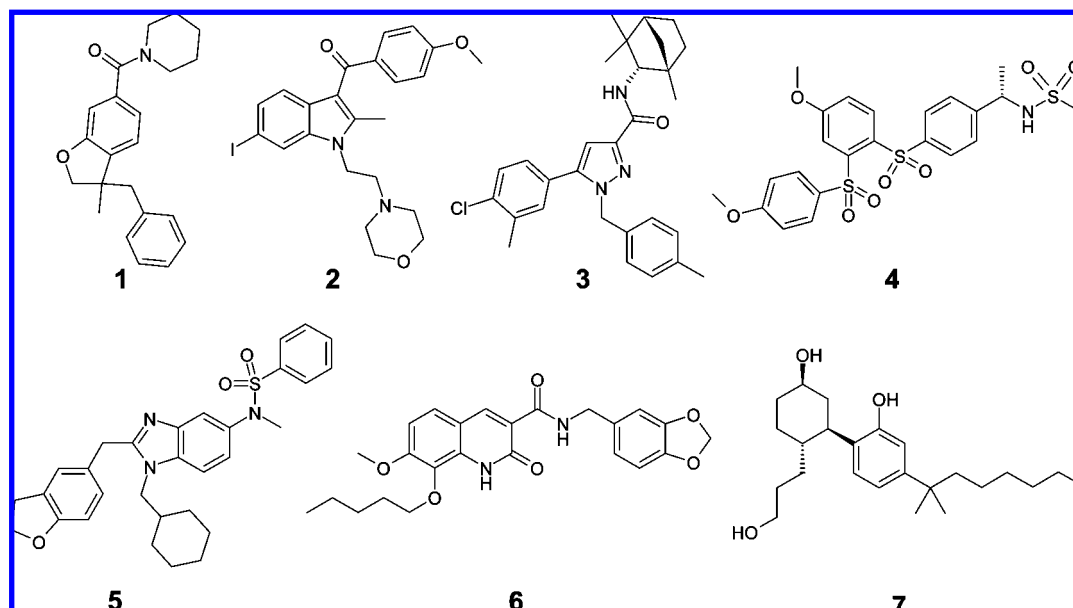
Figure 1. Chemical structures of CB2-selective modulators (1–6) and a nonselective CB agonist (7). (1) MDA7; 10 (2) AM630; 29 (3) SR144528; 27 (4) Sch.336; 36 (5) N -[1-cyclohexylmethyl-2-(2,3-dihydro-1-benzofuran-5-ylmethyl)-1 H -benzimidazol-5-yl]- N -methylbenzenesulfonamide; (6) JTE-907; 30 (7) CP55,940. 77
