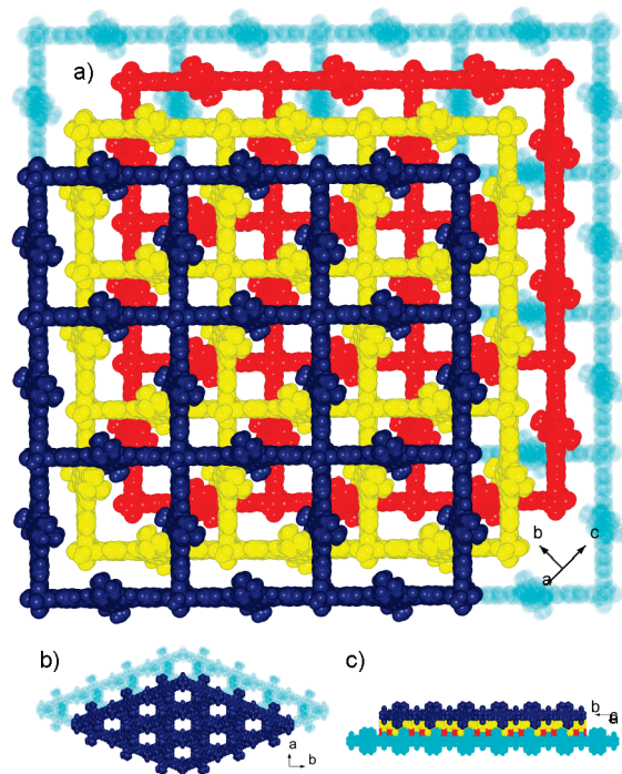
Figure 2. Crystal structures of MAS-1 : (a) space-filling representation of the top view of four square-grid layers showing the distinct openings with various sizes; (b) view of the stacking nets along the c axis; (c) side view of the stacking nets.
