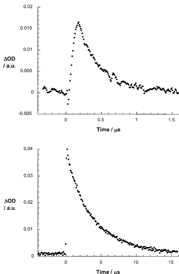
Figure 7. Time-absorption profiles at 1000 nm monitoring the \text{C}_{60}^{\cdot-} decay dynamics in 16 (top) and 20 (bottom) obtained upon nanosecond flash photolysis (355 nm) of approximately 1.0 \times 10^{-5} \text{ M} deoxygenated benzonitrile solutions.
