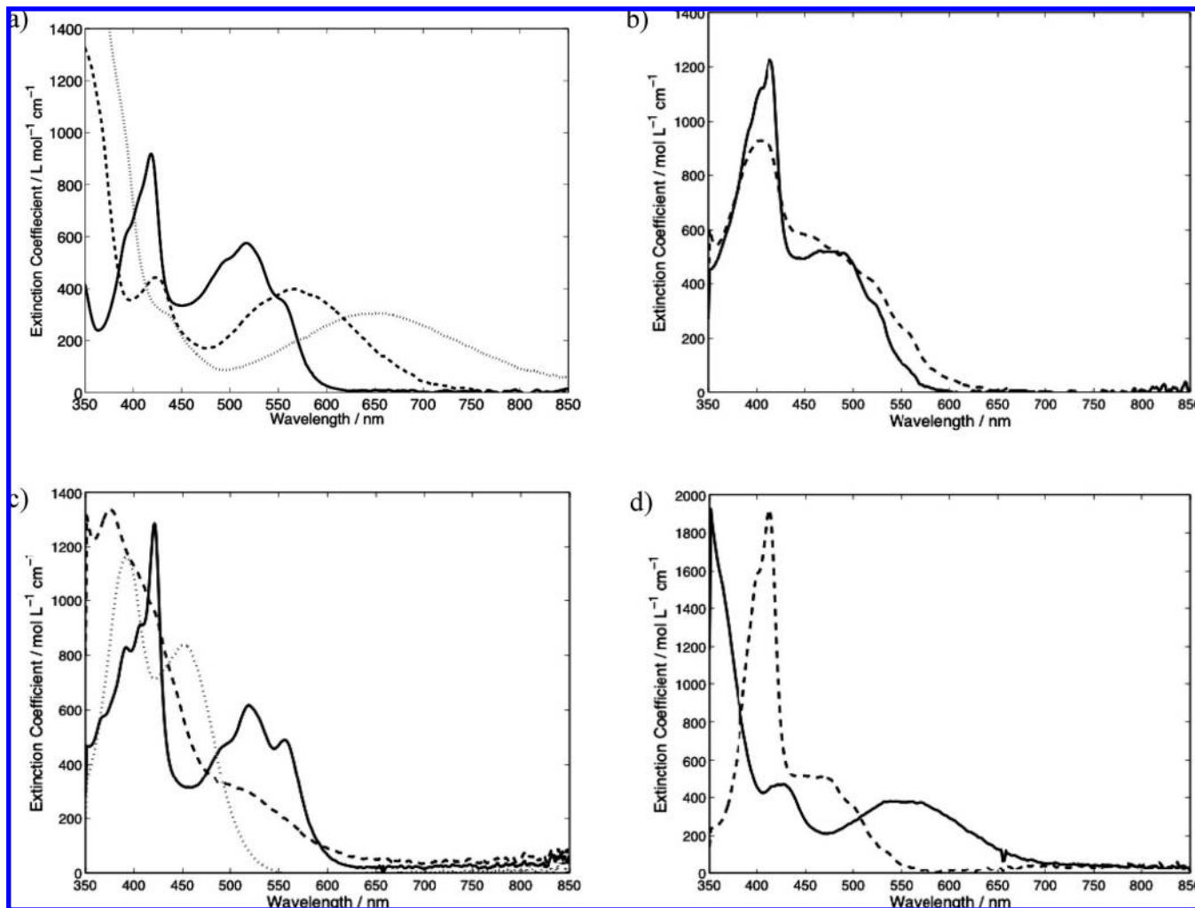
FIGURE 3. (a) UV spectra of 3a (—) and the corresponding anion (---) in 80% aqueous methanol (---) and acetonitrile (···). (b) UV–vis spectra of radical 3b (—) and the corresponding anion (---) in 80% aqueous methanol. (c) UV–vis spectra of radical 3f (—) and the corresponding anion (---) in 80% aqueous methanol and radical 3f in acetonitrile (···). (d) UV–vis spectra of radical 3j (—) and the corresponding cation (---) in 80% aqueous methanol.
