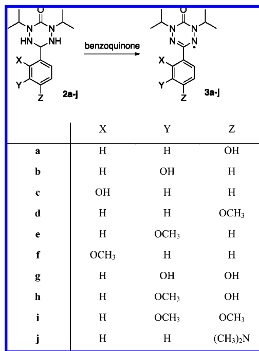
SCHEME 1. Synthesis of Oxophenyl and Aminophenyl-Substituted Verdazyl Radicals
