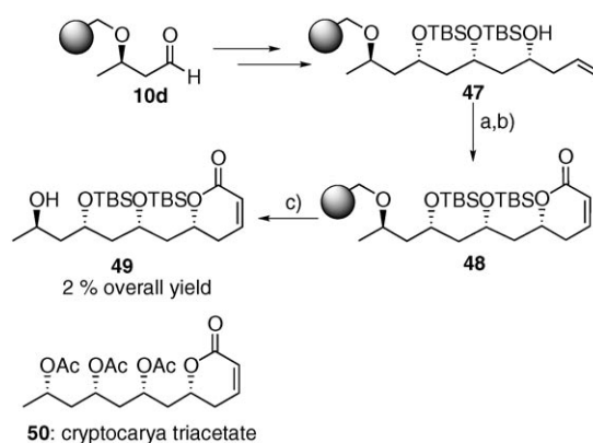
Scheme 5. Synthesis of a diastereomeric analogue of cryptocarya triacetate on a solid support. a) acryloyl chloride, NEt 3 , cat. DMAP, CH 2 Cl 2 , 0 °C to RT, 16 h; b) 19 (2 × 20 mol %), CH 2 Cl 2 , reflux, 24 h; c) DDQ (10 equiv), CH 2 Cl 2 , pH 7 buffer, 0 °C to RT, 16 h.
