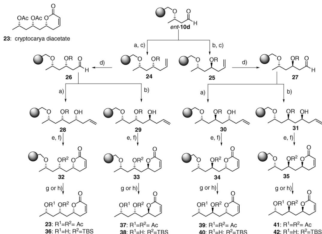
Scheme 4. Stereocomplementary synthesis of all (4' S )-isomers of cryptocarya diacetate. a) i) L -Ipc 2 BAl (3 equiv), THF, −78 °C; ii) pH 7 buffer, H 2 O 2 30%, DMF/MeOH 1:1, 0 °C, 2 h; b) i) D -Ipc 2 BAl (3 equiv), THF, −78 °C; ii) pH 7 buffer, H 2 O 2 30%, DMF/MeOH 1:1, 0 °C, 2 h; c) TBSCl, imidazole, cat. DMAP, CH 2 Cl 2 , RT, 16 h; d) O 3 , CH 2 Cl 2 , −78 °C, then PPh 3 , −78 °C to RT; e) acryloyl chloride, DIPEA, cat. DMAP, CH 2 Cl 2 , 0 °C to RT, 16 h; f) Grubbs second-generation catalyst (2 × 20 mol %) ( 18 ), CH 2 Cl 2 , reflux, 24 h; g) i) trifluoroacetic acid/CH 2 Cl 2 1:2, 20 min, RT; (ii) Ac 2 O, NEt 3 , cat. DMAP, CH 2 Cl 2 , 0 °C to RT, 3 h; h) DDQ (10 equiv), CH 2 Cl 2 , pH 7 buffer, 0 °C to RT, 16 h; DIPEA = diisopropyl ethyl amine.
