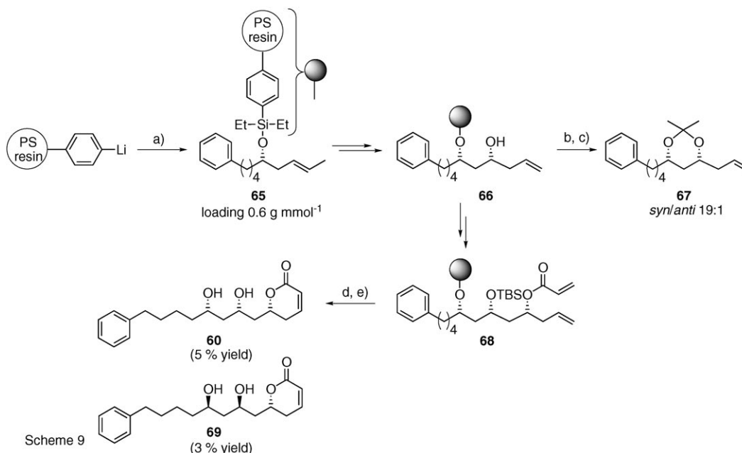
Scheme 9. Synthesis of natural-product-derived compounds on a diethylsilylpolystyrene resin. a) i) Et 2 SiCl 2 (6 equiv), THF, 0°C to RT, 2 h; ii) (5 S ,2 E )-5-hydroxy-9-phenyl-non-2-ene (3 equiv), 2,6-lutidine (3 equiv), DMAP (0.5 equiv), CH 2 Cl 2 , RT, 16 h; b) HF/pyridine, pyridine, THF, RT, 8 h; c) 2,2-dimethoxypropane, cat. (+)-CSA; d) 19 (2 × 20 mol %), CH 2 Cl 2 , reflux, 24 h; e) HF/pyridine, pyridine, THF, 40°C, 16 h. CSA = camphorsulfonic acid.
