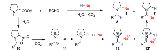
Figure 1. Proposed mechanism for the reaction of azomethine ylides with pronucleophiles.
