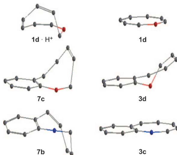
Fig. 6. Calculated equilibrium geometries of anions 1d , 3c , and 3d , and their respective conjugate acids 1d \cdot H^+ , 7b , and 7c
