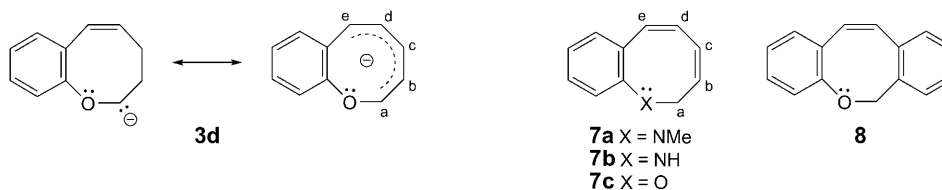
Fig. 3. 2H -1-Benzoxocin-2-ide ( 3d ), 2H -1-benzheterocins 7a–7c , and 6H -dibenz[ b,f ]oxocin ( 8 )
