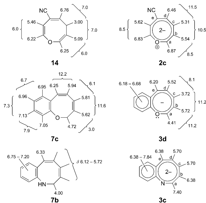
Fig. 4. ^1\text{H} -NMR Data ( \delta in ppm, J in Hz) for Anions 2c , 3c , 3d , and the corresponding conjugate-acid precursors 14 , 7b , and 7c . For convenience, the H-atoms at the cyclic structures are represented by their bonds (without attached H).
