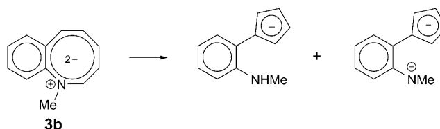
Scheme 3. Rearrangement of 1-Methyl-1-benzazocin-2(1H)-ide Anion ( 3b )
