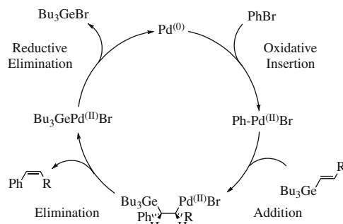
Scheme 2. Proposed mechanism.
