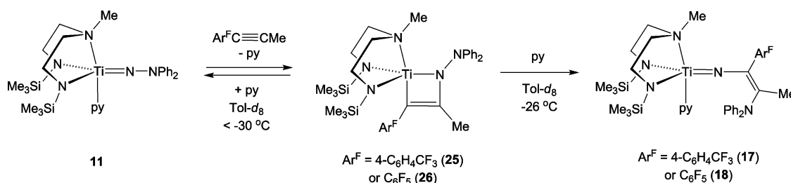
Scheme 3. Reaction of \text{Ti}(\text{N}_2\text{N}^{\text{Me}})(\text{NNPh}_2)(\text{py}) ( 11 ) with \text{Ar}^{\text{F}}\text{CCMe} ( \text{Ar}^{\text{F}} = 4\text{-C}_6\text{H}_4\text{CF}_3 or \text{C}_6\text{F}_5 )
