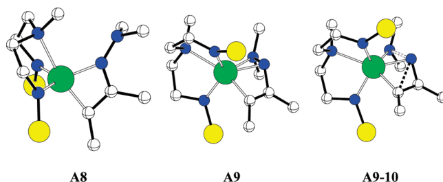
Figure 9. Optimized geometries for the azatitanacyclobutene A8 , the N β Me 2 -chelated intermediate A9 , and the TS for N α –N β cleavage ( A9 – 10 ). H atoms have been omitted for clarity.
