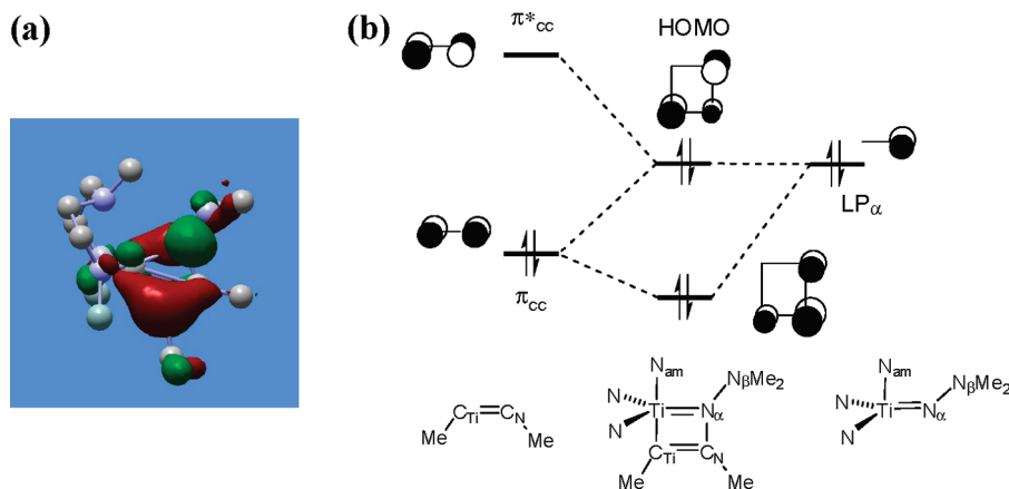
Figure 8. (a) HOMO of A8 . (b) Schematic MO diagram for the \pi interactions within the 4-membered metallacycle
