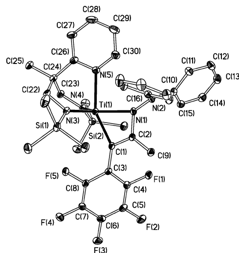
Figure 2. Displacement ellipsoid plot (25% probability) of Ti(N_2N^{py})\{N(NPh_2)C(Me)C(C_6F_5)\} ( 4 ). H atoms omitted for clarity. Selected distances (Å): Ti(1)-N(1) 2.119(2), Ti(1)-N(3) 1.895(2), Ti(1)-N(4) 1.902(2), Ti(1)-N(5) 2.232(2), Ti(1)-C(1) 2.065(2), N(1)-N(2) 1.418(2), N(1)-C(2) 1.382(3), N(2)-C(10) 1.398(2), N(2)-C(16) 1.416(2), C(1)-C(2) 1.378(3), C(1)-C(3) 1.448(3).
