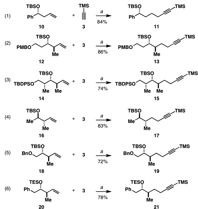
Figure 2. Formal hydroalkynylation by alkynylborate chemistry.
