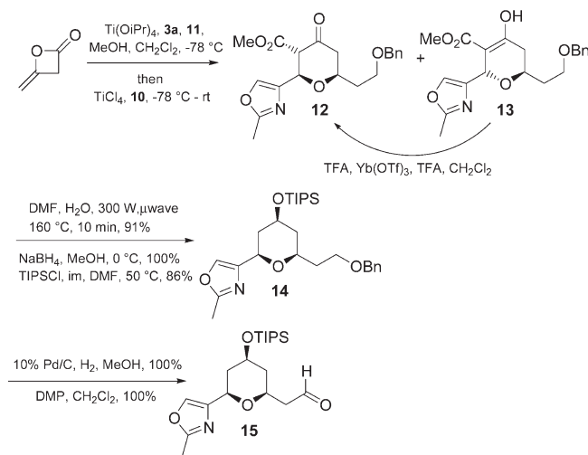
Scheme 3. Synthesis of the First Tetrahydropyran 15
