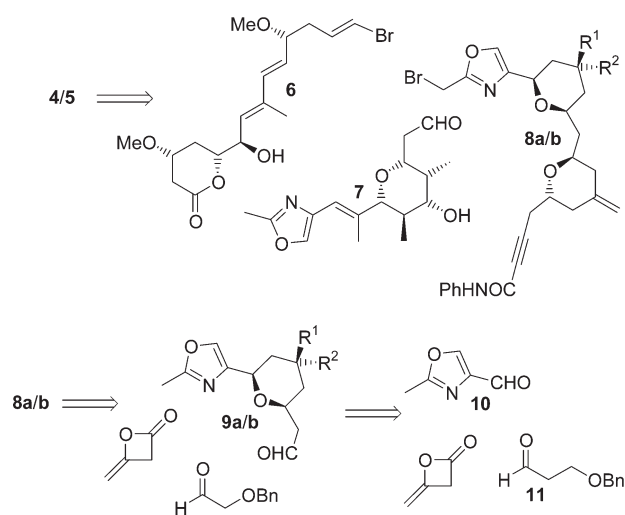
Scheme 2. Retrosynthetic Analysis of the Bis -pyran Units of the Phorboxazoles
