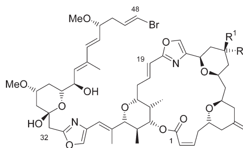
Figure 1. Phorboxazole A, 4 : \text{R}^1 = \text{H}, \text{R}^2 = \text{OH} ; phorboxazole B, 5 : \text{R}^1 = \text{OH}, \text{R}^2 = \text{H} .
