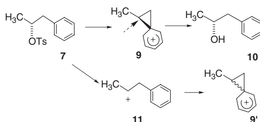
Scheme 3. Hydrolysis of 7 via benzenium ion 9 and formation of racemic benzenium 9' .
