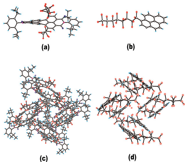
Figure 1. Molecular structure of 3b (a) and 13 (b). Crystal packing of 3b (c) and 13 (d).
