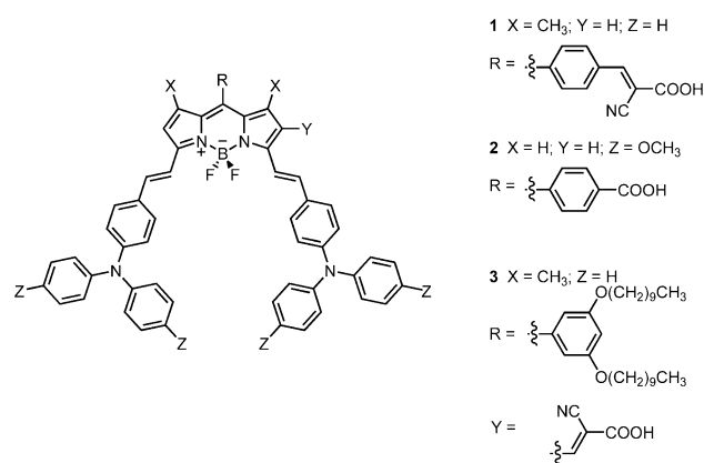
Figure 1. Sensitizers used in this study.
