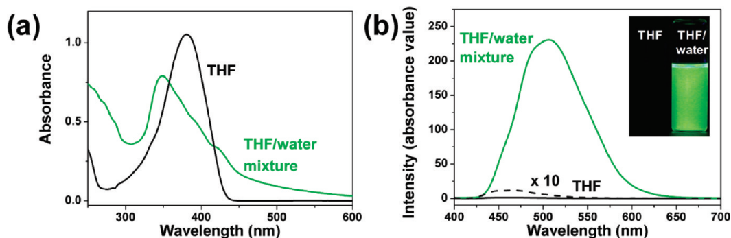
Figure 1. (a) UV–visible absorption spectra of DBDCS in THF solution ( c = 2 \times 10^{-5} mol L ^{-1} , black line) and DBDCS nanoparticles in THF/water mixture ( c = 2 \times 10^{-5} mol L ^{-1} , green line). (b) PL spectra of DBDCS in THF solution (black line) and DBDCS nanoparticles in THF/water mixture (green line). Insets show the fluorescence images of DBDCS in THF solution and DBDCS nanoparticles in THF/water mixture under 365 nm UV light.
