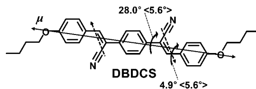
Scheme 1. Molecular Structure of DBDCS and Its Local Dipoles (dashed arrows) and Transition Dipole Moment \mu(S_0 \rightarrow S_1) (double arrow, the length of 12.6 D) and Dihedral Torsional Angles in Isolated State and Single Crystal State (in brackets)
