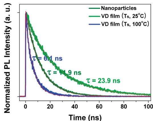
Figure 7. Fluorescence decay profiles of DBDCS nanoparticles in THF/water mixture (dark green line), G -phase VD film (green line), B -phase VD film (blue line) under 400 nm excitation. Red lines are the best fitting curves.
