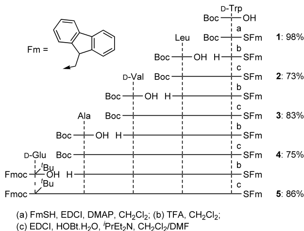
Scheme 2. Typical Synthesis of a seco -Thioester for Cyclization
