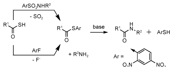
Scheme 1. Amide Formation from Thioacids with either Sulfonamides or Amines and Sanger's Reagent
