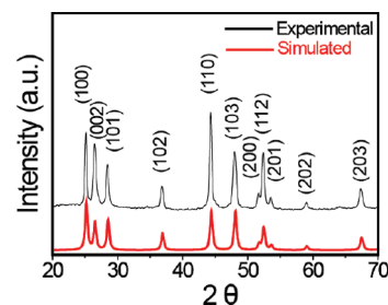
Figure 1. Experimental and simulated XRD patterns of CISE NCs with a wurtzite structure.
