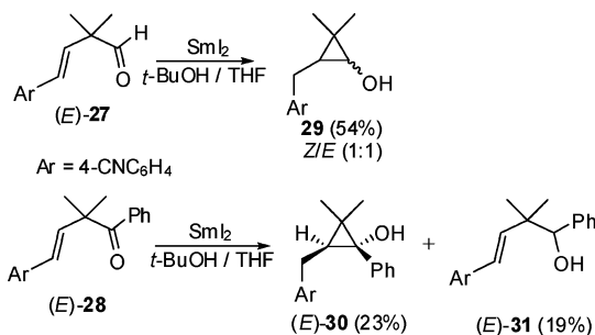
Scheme 7. SmI 2 -Mediated 3- exo-trig Cyclization of 4-Cyanophenyl-Substituted Compounds 27 and 28
