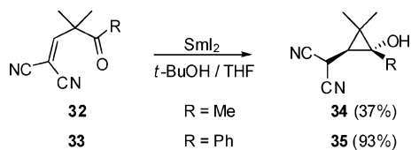
Scheme 8. SmI 2 -Mediated 3- exo-trig Cyclization of Dicyano-Substituted Ketones 32 and 33
