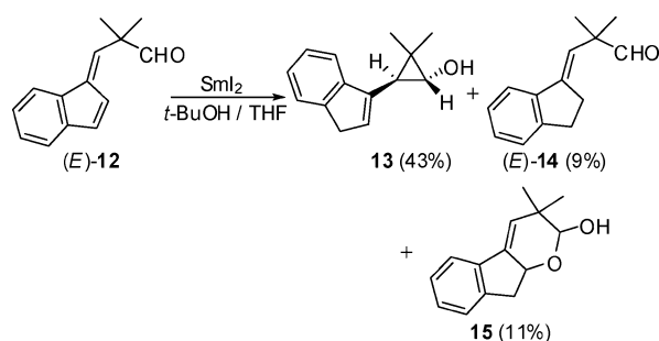
Scheme 3. Treatment of Aldehyde 12 with \text{SmI}_2
