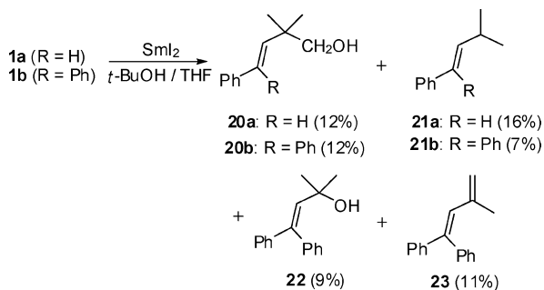
Scheme 5. Treatment of Aldehydes 1 with \text{SmI}_2
