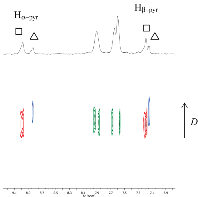
Figure 4. ^1\text{H} -DOSY NMR spectrum of 4a/4b in \text{CD}_2\text{Cl}_2 at 223 K.
