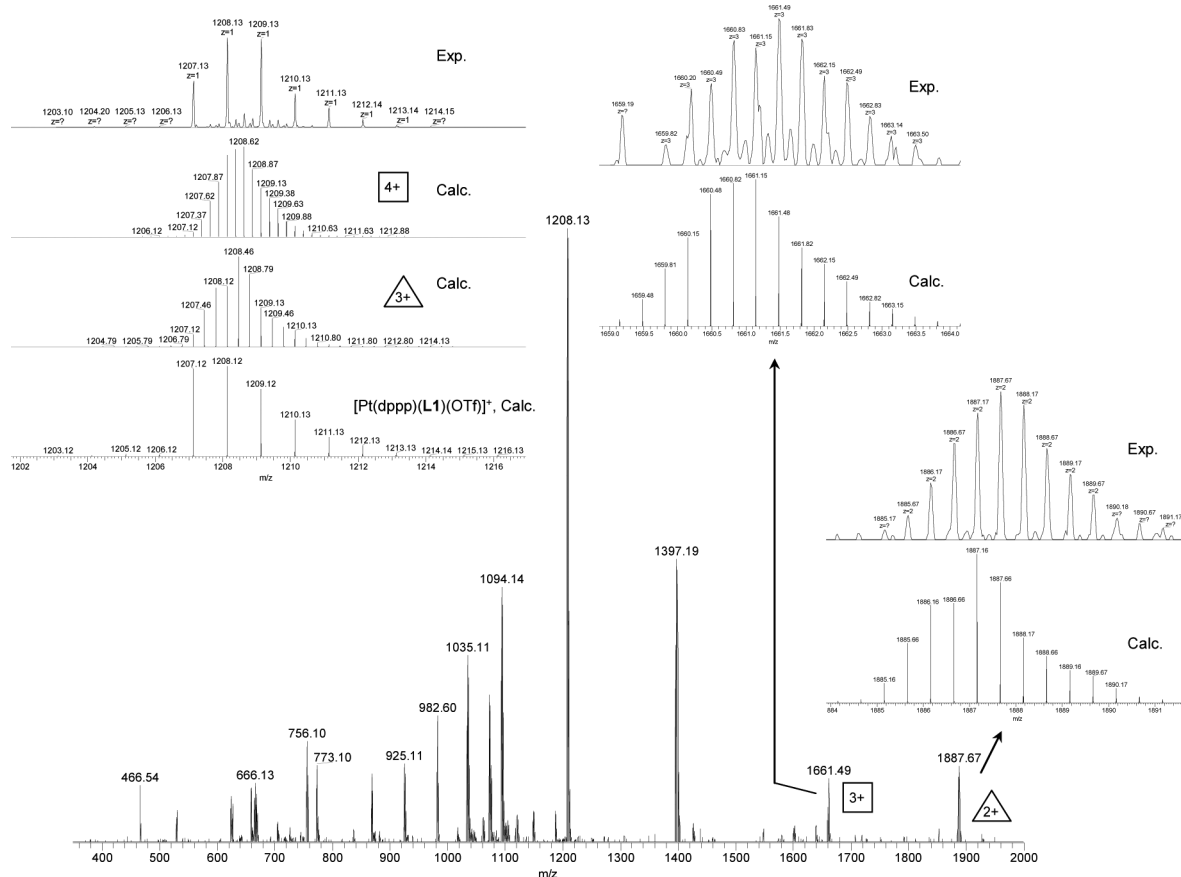
Figure 3. ESI-MS spectrum of 2a/2b in acetone.
