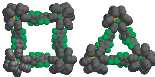
Figure 5. Minimum energy geometry calculated for compound 4a (left) and 4b (right) (hydrogens are omitted for clarity).
