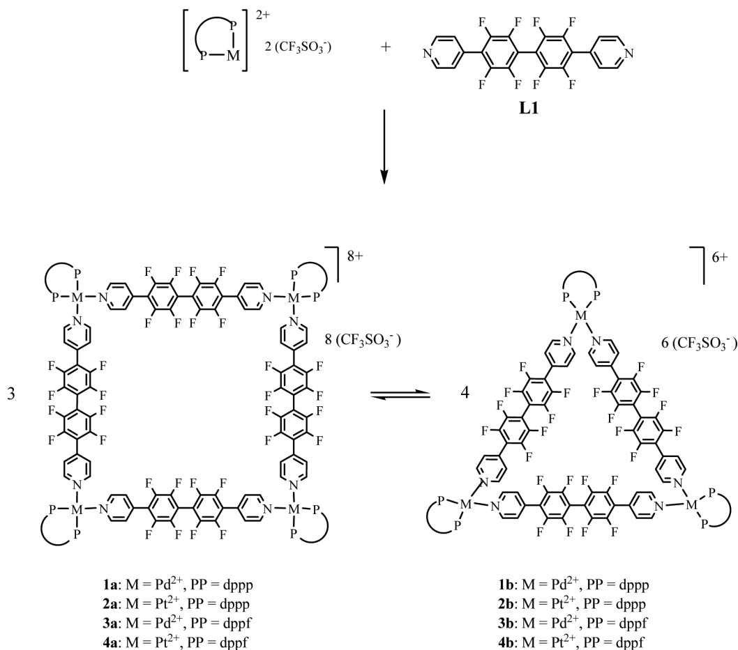
Scheme 2. Self-Assembly Reactions between L1 and the Diphosphane Metal Corners
