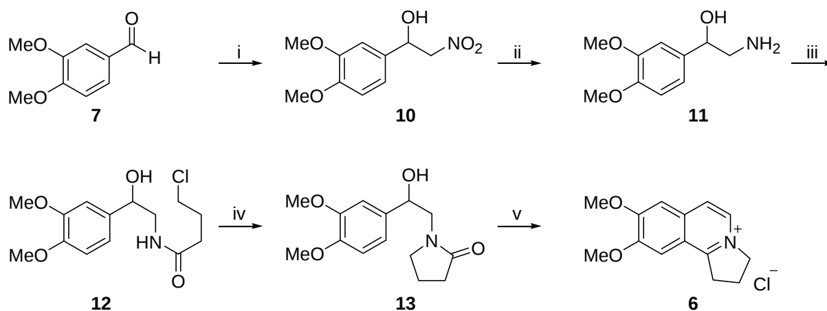
Scheme 2. Reagents and conditions: i MeNO 2 ( 8 ), MS4A, DMSO, rt, 24 h, 86%; ii H 2 , Pd-C, EtOH, rt, 2 h; iii Cl(CH 2 ) 3 COCl ( 9 ), TEA, CHCl 3 , 0 °C, 2 h, 93% (2 steps), iv NaH, DMF, 0 °C, 3 h, 85%; v POCl 3 , toluene, reflux, 3.5 h, 81%
